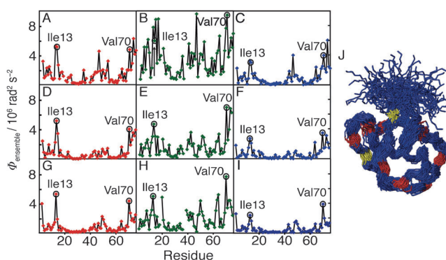
Figure 2. Predicted chemical shift variance ( \Phi_{ensemble} ) of EROS (A, B, and C), EROSII (D, E, and F) and ERNST (G, H, and I) ensembles. Chemical shifts were extracted from the ensemble members ( N = 116 for EROS, N = 176 for EROSII, N = 640 for ERNST) with the programs SHIFTX (A, D, and G; red), SHIFTS (B, E, and H; green), and SPARTA (C, F, and I; blue). Residues Ile13 and Val70 showing consistently the largest \Phi_{ensemble} through all ensembles and all programs are indicated. The EROS ensemble (J) labelled with the RD detected residues, Ile13 and Val70 (yellow) and the eight residues with higher supra- \tau_c mobility (red).
