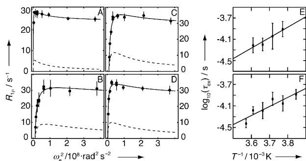
Figure 1. Temperature-dependent relaxation dispersion. R_{1\rho} dispersion curves measured at -8^\circ C for residues Ile13 (A), Ile23 (B), Asn25 (C), and Val70 (D) plotted as a function of the rotating frame effective field. Solid and dashed lines represent the nonlinear fit to the data and the exchange contribution extracted from the fit, respectively. Arrhenius-type fit to the temperature-dependent RD exchange rates (see Table S1 in the Supporting Information) for Ile13 (E) and Val70 (F). Activation energies of (37 \pm 7) kJ mol^{-1} and (32 \pm 8) kJ mol^{-1} were extracted for Ile13 and Val70, respectively.
